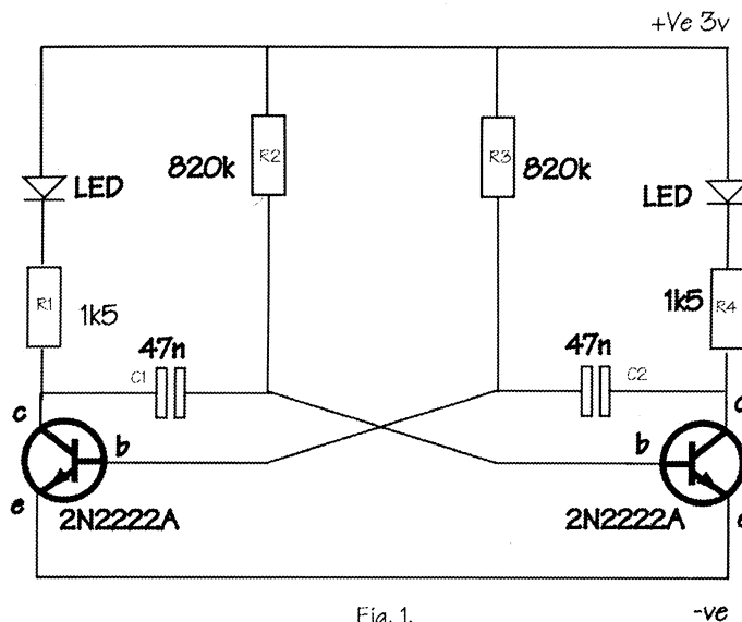
Fig. 1. Astable multivibrator
